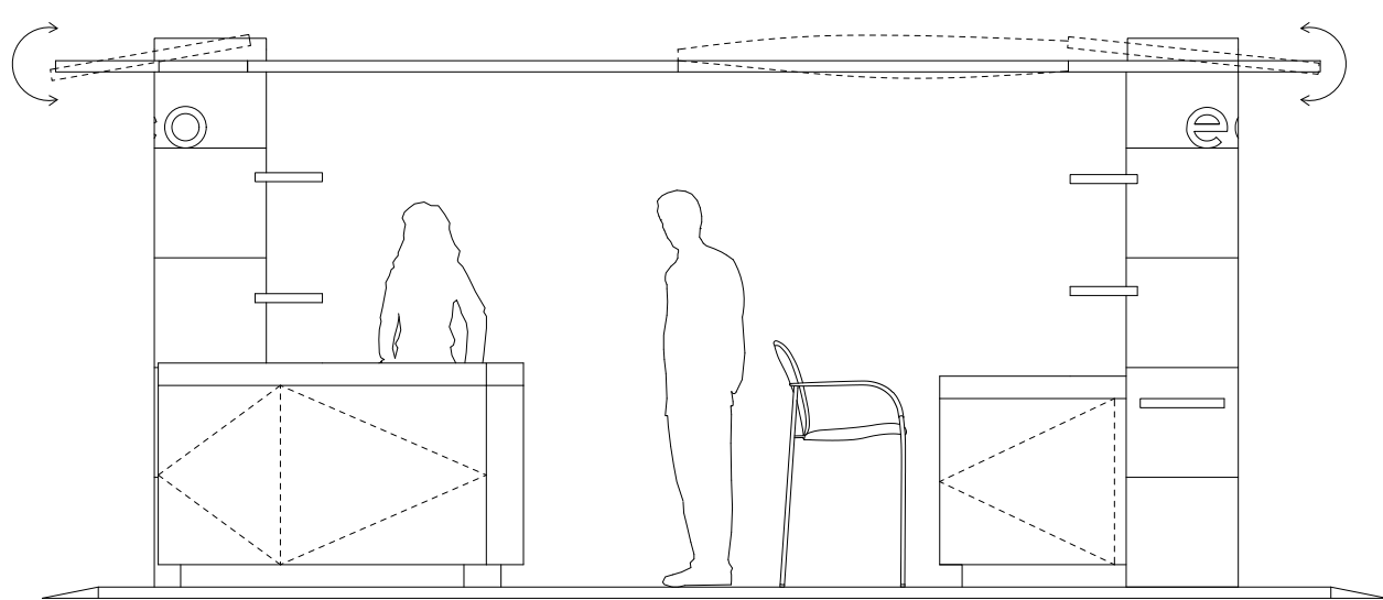
SIDE ELEVATION
